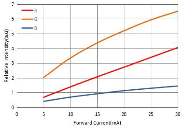
Figure4. Typical normalized light output vs. forward current
