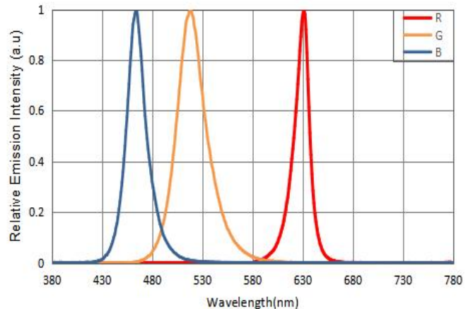
Figure6. Color Spectrum, Tj = 25°C, IF=20mA
