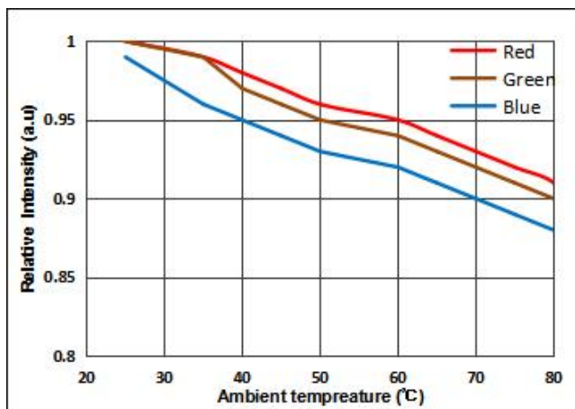
Figure5. Relative Intensity Vs. Ambient Temperature
