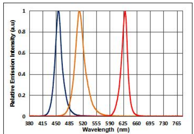
Figure6. Color Spectrum, Tj = 25°C, IF=20mA
