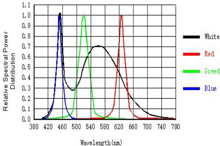
Figure6. Color Spectrum, Tj = 25°C, IF=150mA
