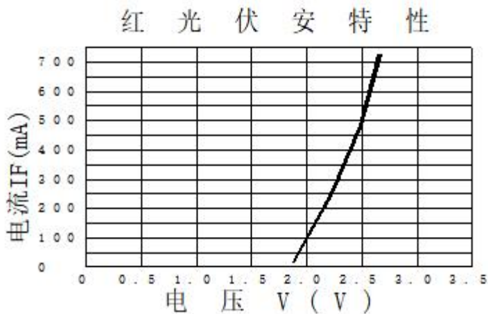
Figure4. Typical forward current vs. forward voltage
