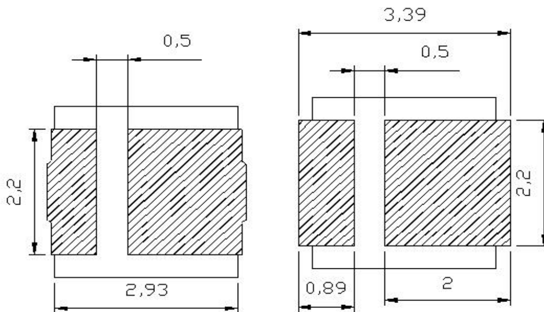
Recommended Copper Layout
