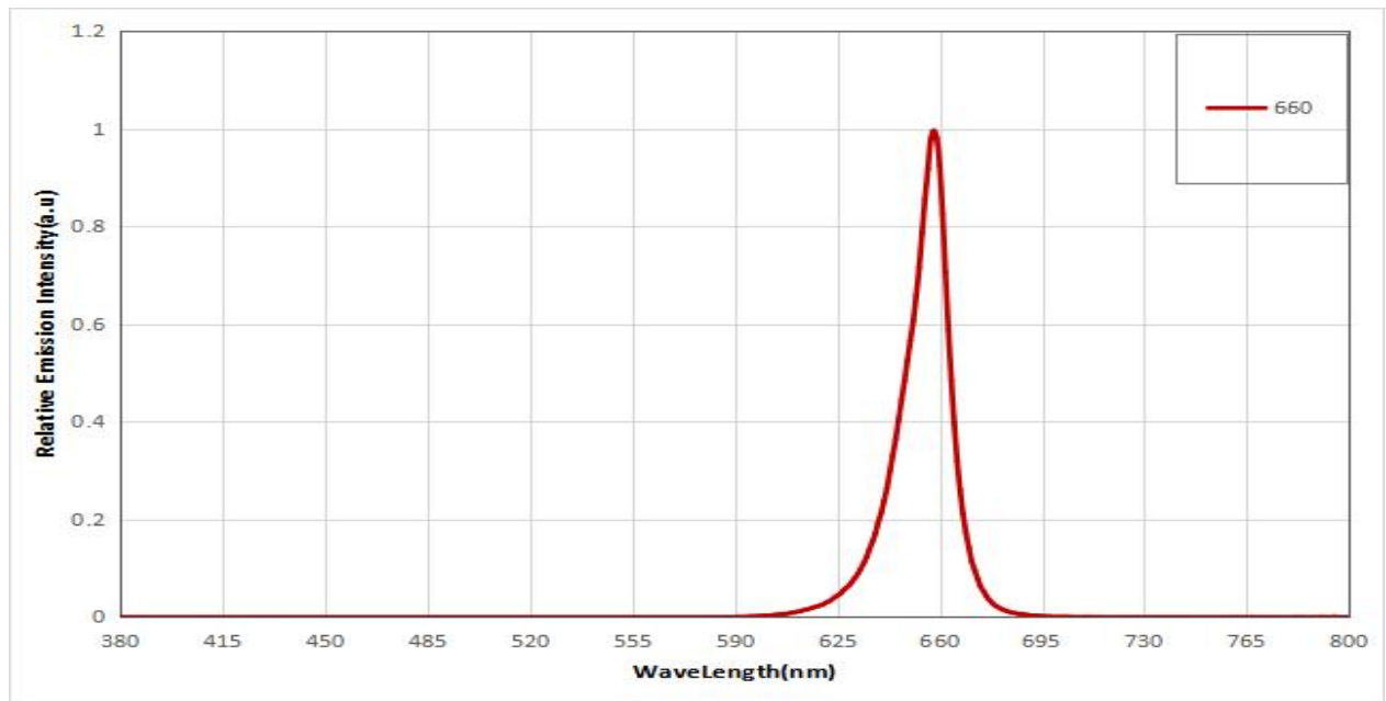
Figure1. Typical normalized power vs. wavelength for Red
