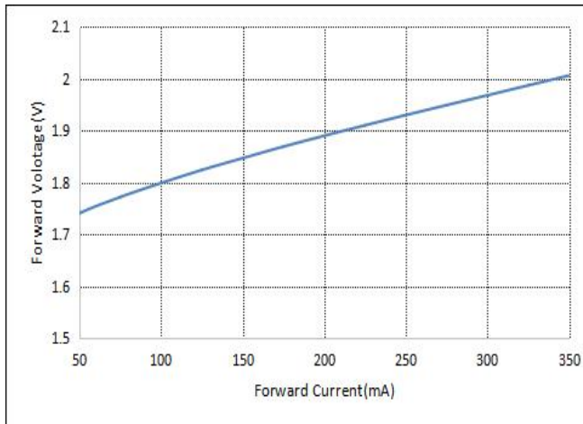
Figure3. Typical forward current vs. forward voltage
