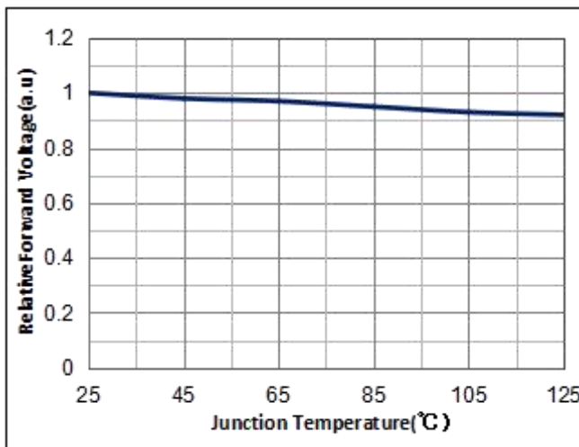
Figure5. Forward Voltage Vs. Case Temperature
