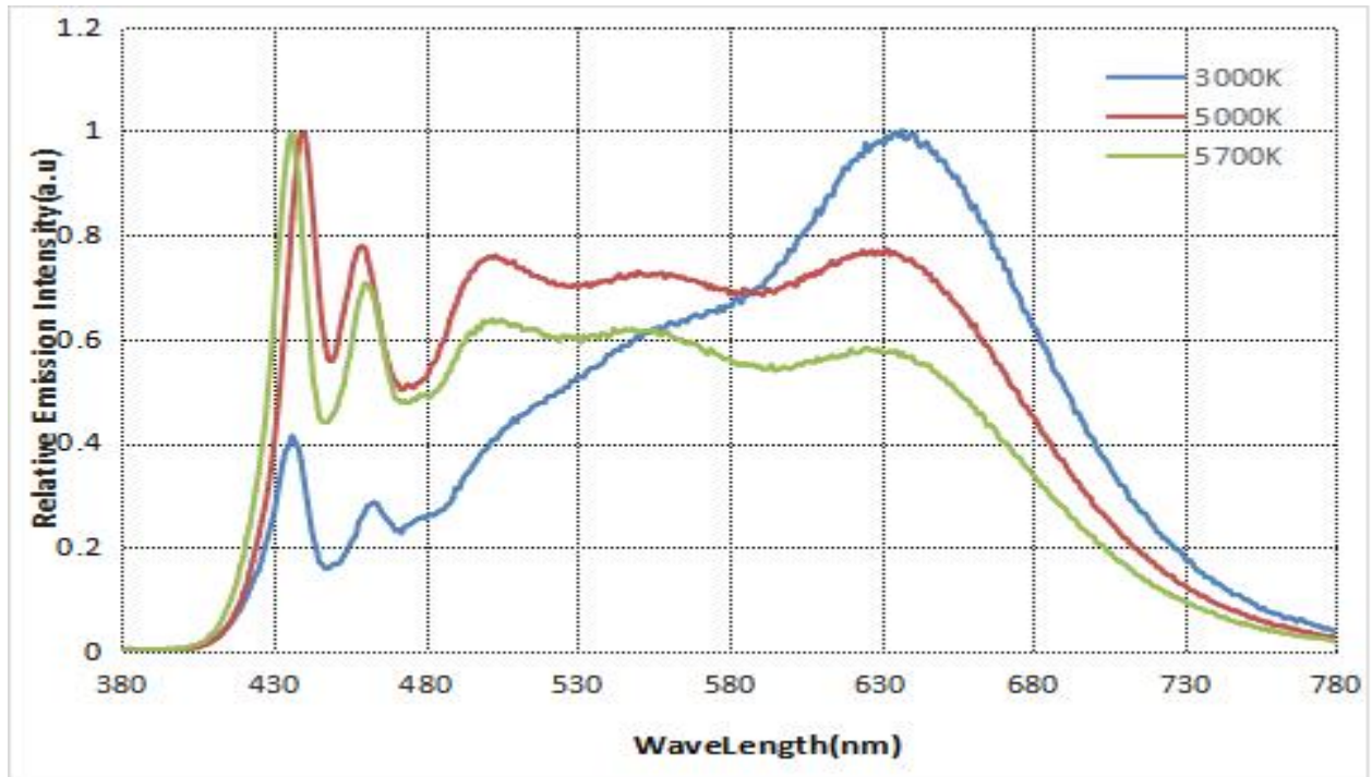
Figure1. Typical normalized power vs. wavelength for 95CRI
