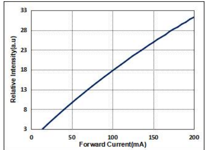
Figure4. Typical normalized light output vs. forward current
