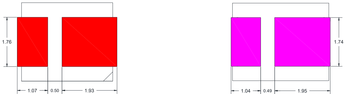
Recommended Copper Layout
